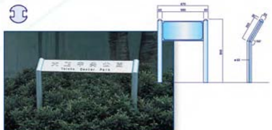
Module Plus post ø 60mm with 1 standard 250 mm deep text panel
